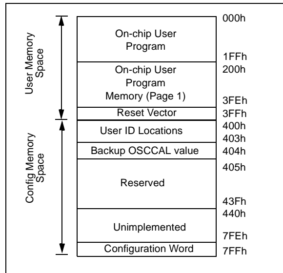
FIGURE 2-1: PIC16F505 PROGRAM MEMORY MAP
