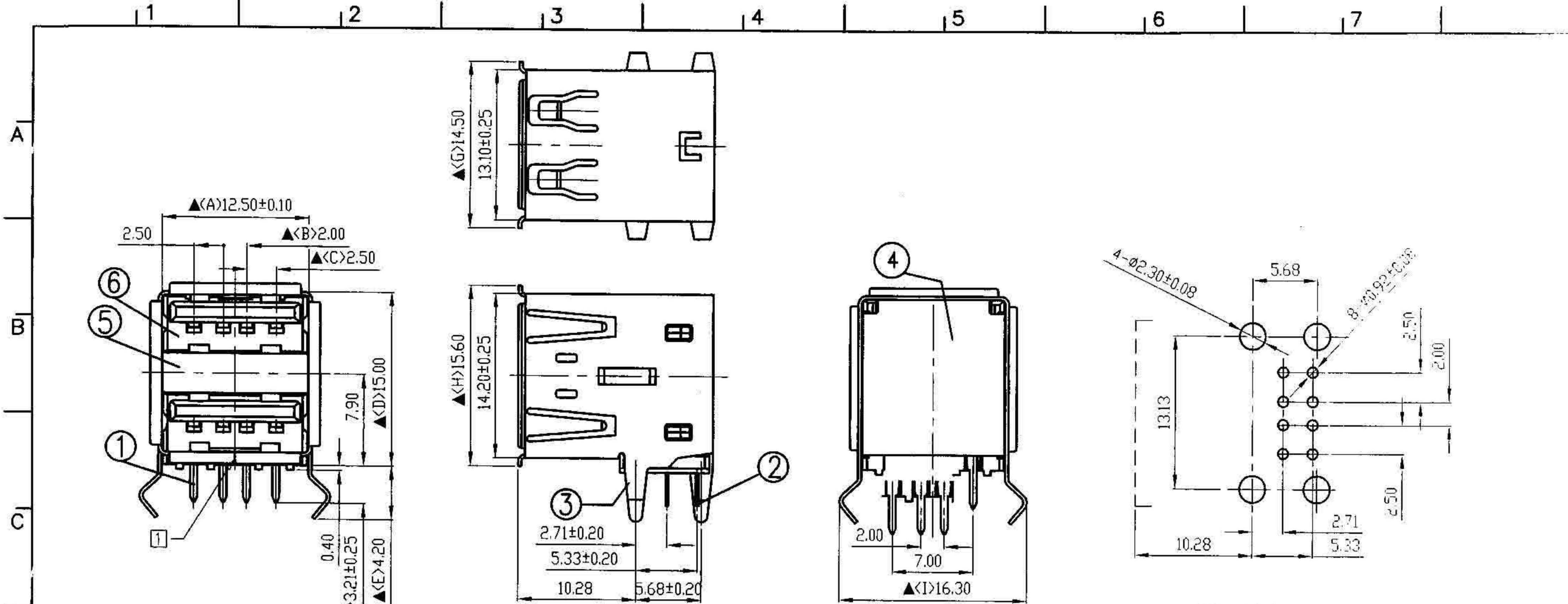
Pin Hole Layout (Jack Bottom View)
