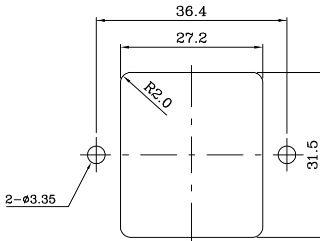
PANEL CUT-OUT
