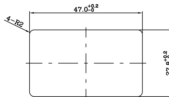
PANEL CUT-OUT
