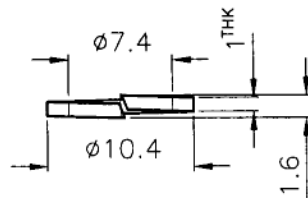
SPRING WASHER
